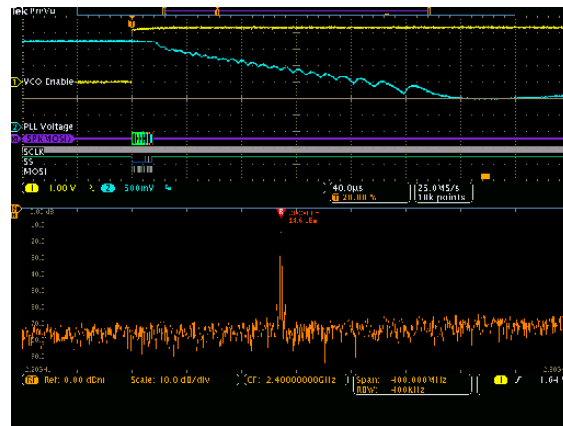
3. Spectrum Time is moved another 160 \mu s to the right. At this point the spectrum shows that the PLL has actually overshoot the correct frequency and gone all the way down to 2.388 GHz.
